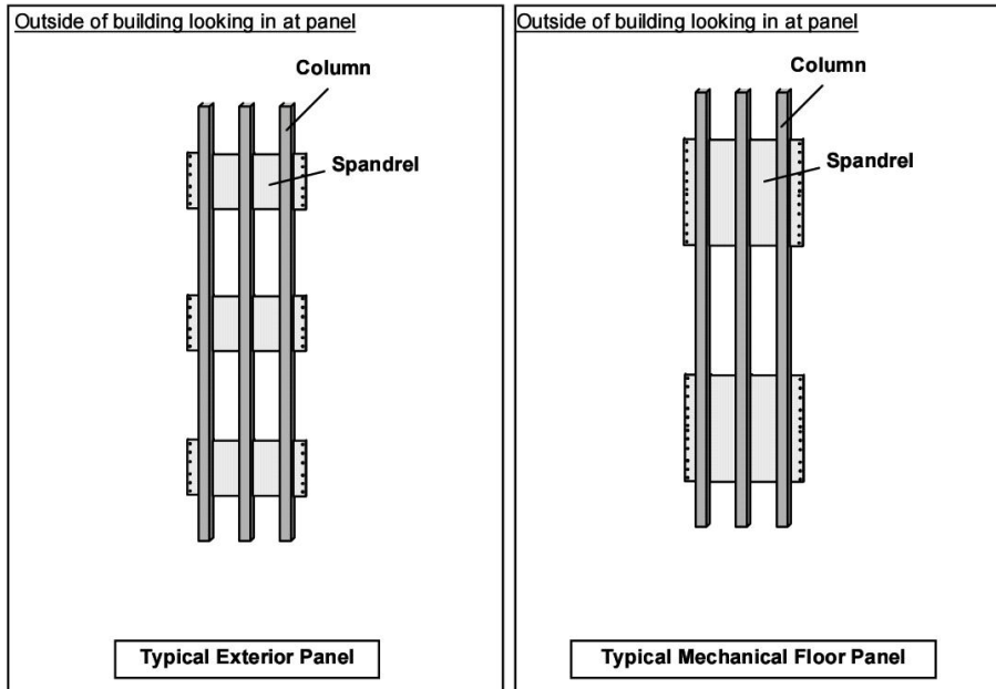
Figure 1-1 Spandrels – “Wheatchex” - Page 27 of NCSTAR1-3B
