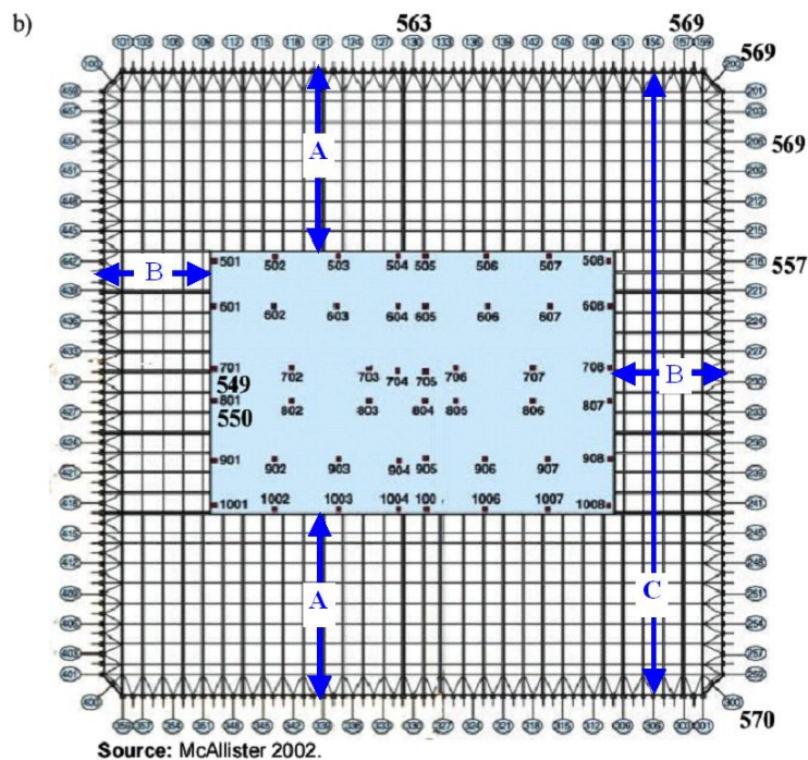
Figure 1-2 Diagram Illustrating Total Lengths of Truss Steel (Page 16 of NCSTAR1-3B)
