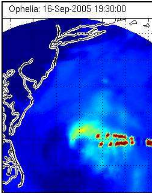
Figure 174 - Hurricane Ophelia - Wisconsin University MIMIC recording.
