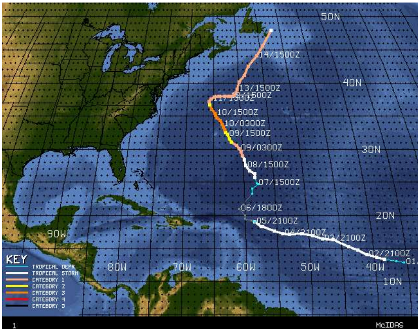
Figure 172 – Path of Hurricane Erin – 01 to 14 September 2001
