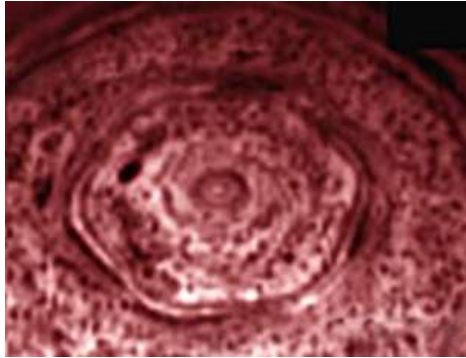
Figure 22 – an early photo of Saturn’s hexagonal feature at the North Pole. (The Cassini probe has since photographed this in high resolution.)
