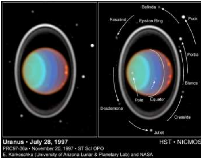
Figure 25 – Storms on Uranus, 1997
