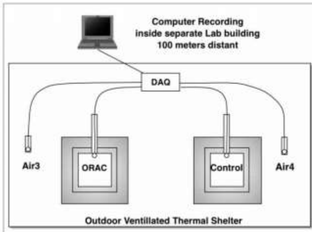
Figure 155 – De Meo’s ORAC reproduction: General layout of the To-T Experiment. Thermistors measure the temperature in the upper interior of both ORAC and Control enclosures, with separate air temperature measurements.
