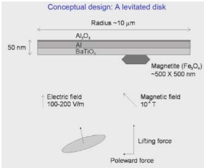
Figure 5 – David Keith’s levitated reflective nano disk.
