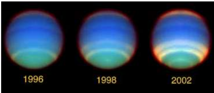
Figure 28 - Alternative image of Neptune in late 1990s/early 2000s
