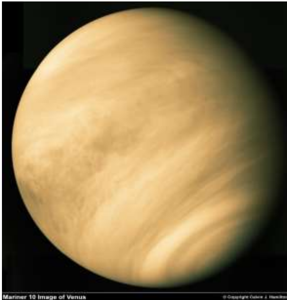
Figure 14 - Venus – composite Mariner 10 image
