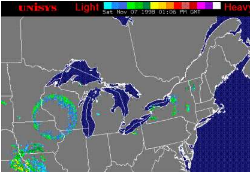
Figure 113 - US Radar Anomaly 07 November 1998
