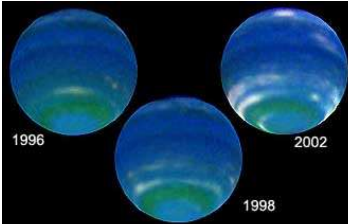
Figure 27 - Bright clouds appear on Neptune in late 1990s/early 2000s
