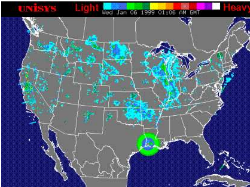
Figure 115 - US Radar Anomaly 06 January 1999
