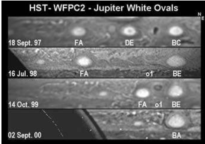
Figure 18 – Images from the Hubble Space Telescope show that between 1997 and 2000, two of Jupiter’s three White Ovals disappeared. UC Berkeley’s Philip Marcus predicts that the disappearance of these storm systems will be followed by a global climate shift on Jupiter within the next decade. (Images courtesy NASA)
