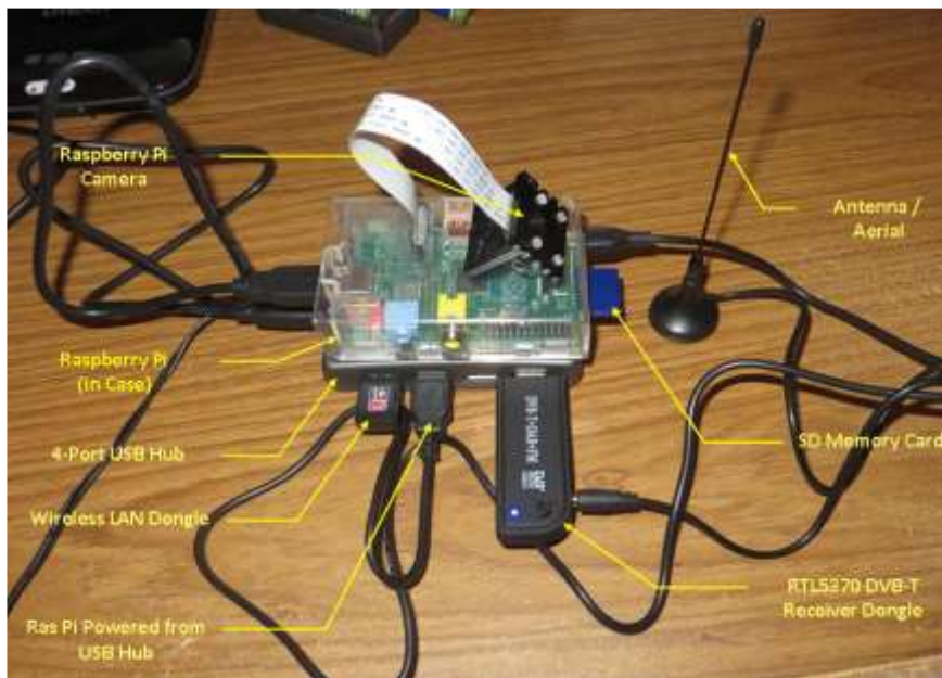
Figure 83 – Single PiTracker in operation.
