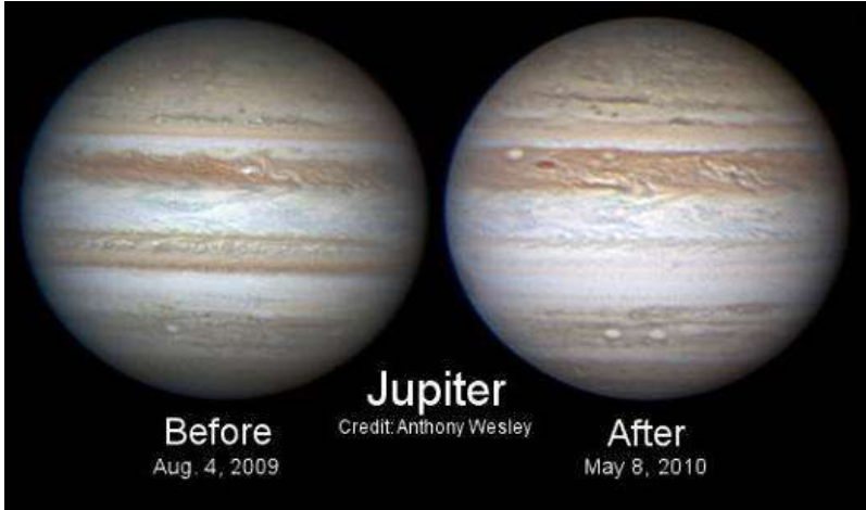
Figure 21 – 20 May 2010 – “Jupiter Loses a Stripe”
