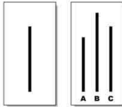
Figure 1 - Asch Conformity experiment - example diagram.
