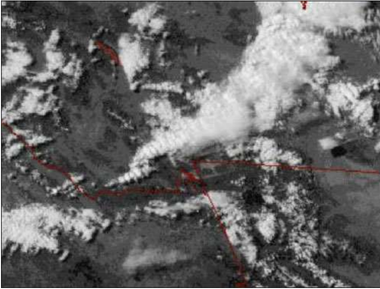
Figure 128 - Satellite image - June 7, 2004-0108Z Southern Montana/East Idaho/NW Montana.
