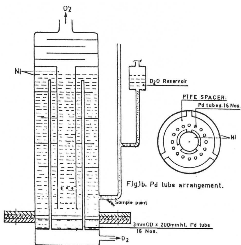
Fig. 1. Schematic View of Milton-Roy Commercial Electrolyzer
