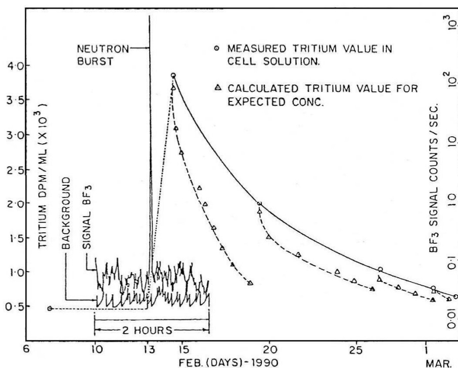
Fig. 7. Neutron and Tritium Output of RCS-11 Experiment
